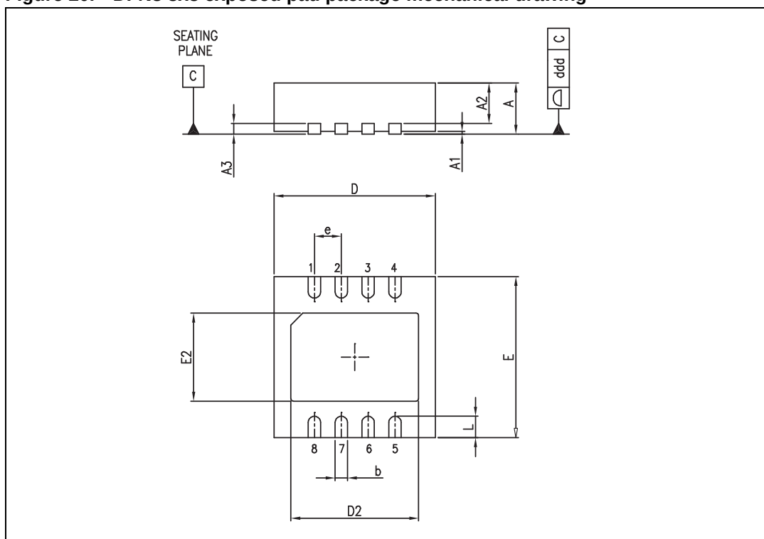
Figure 20. DFN8 3x3 exposed pad package mechanical drawing
