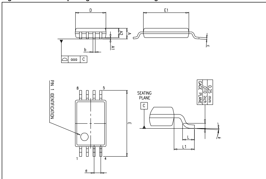
Figure 16. TSSOP8 package mechanical drawing
